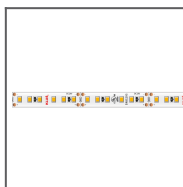
LED-Band K-1220-24V 9.6W/m Ref: K-1220-24V
